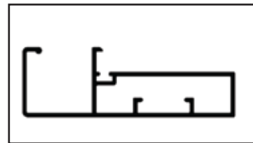
G-Handle (68mm)
